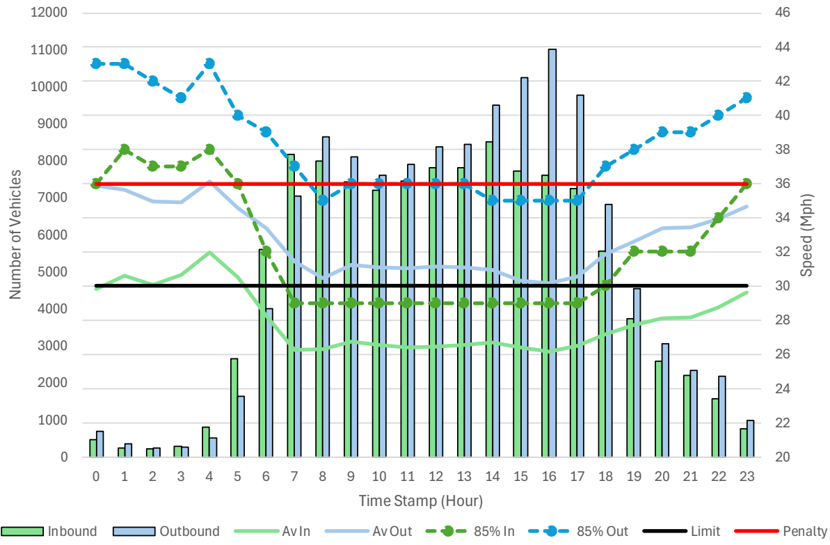
Bradbury Lane - Traffic Volume per Hour with Average Speed and 85% Percentile
