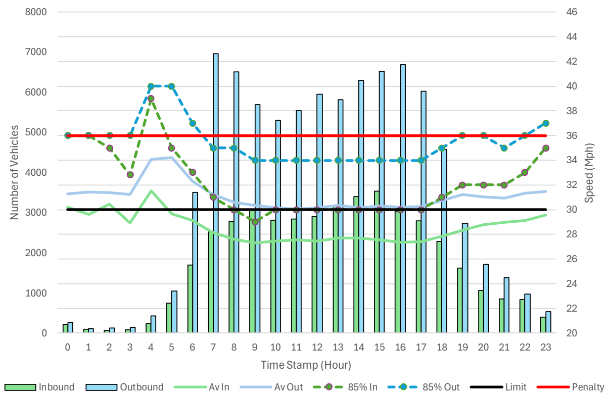
Leofric Close - Free Flowing Traffic Volume, Average Speed and 85% Percentile Speed
