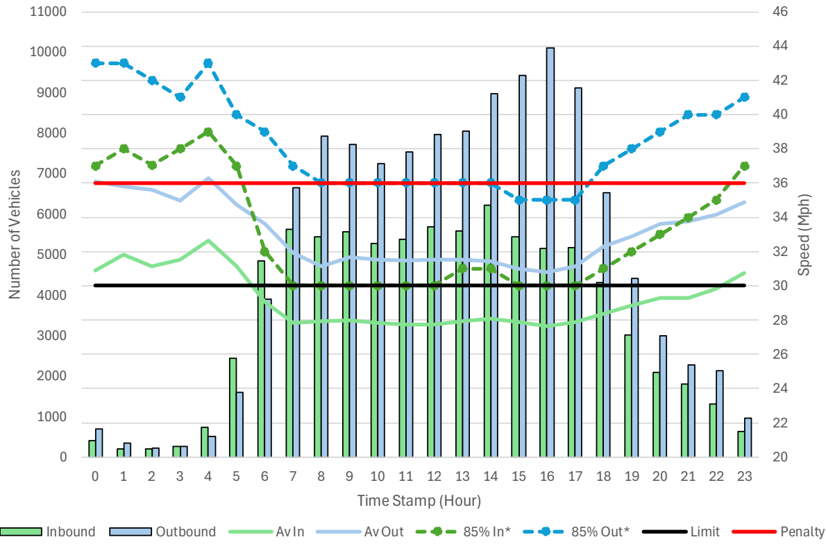
Bradbury Lane - Free Flowing Traffic Volume, Average Speed and 85% Percentile Speed
